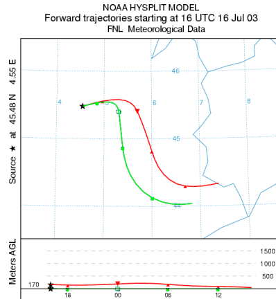
Plume Trajectories for a release centred at 45.48 North and 4.55 East – 16 July 2003 – the location of the incident is shown thus ★
