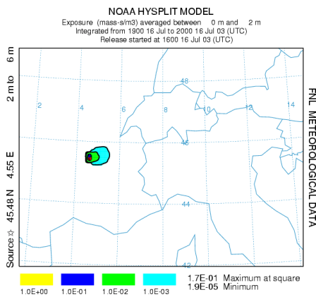
Plume Trajectories for a release centred at 45.48 North and 4.55 East – 16 July 2003 – the location of the incident is shown thus ★
